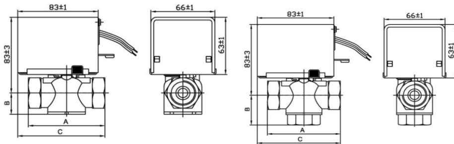
Fig. 2: 3-way Valve
